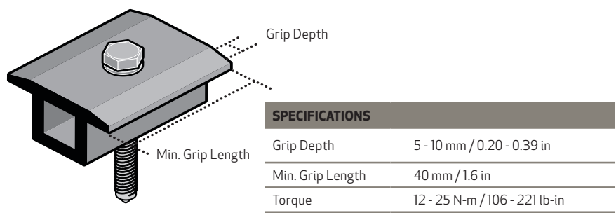
Fig. 1-1 Clamp Specifications
