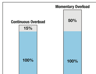
Figure 31 - WEG motor overload capacity
