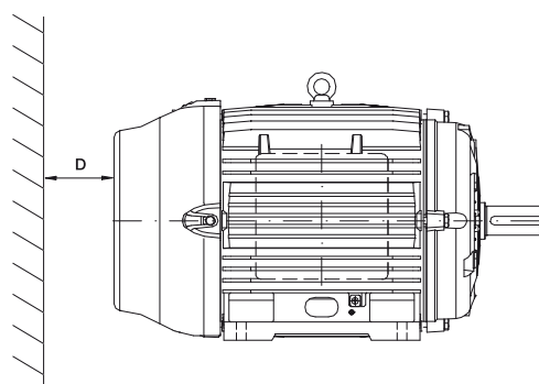
Figure 40 - Minimum distance to wall
