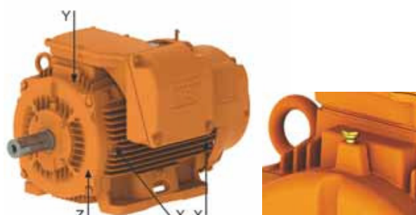
Figure 7 - Flat surfaces for vibration checking (frames 225 to 355)
