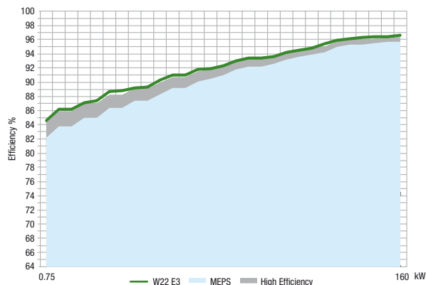
Figure 2 - Typical efficiency curve of W22 line
