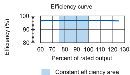
Figure 2 - Typical efficiency curve of W22 line
