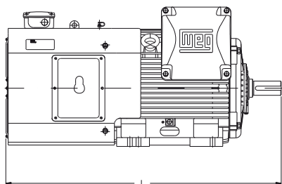
Figure 39 - Forced ventilation kit for W22 motors
