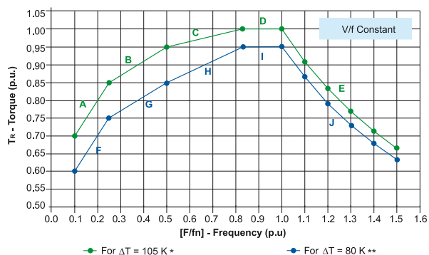
Figure 37 - Derating curve for constant torque
