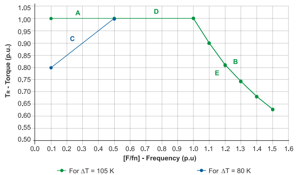
Figure 38 - Derating curve with Optimal Flux®
