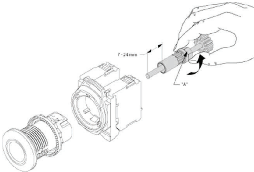
Dimension Diagram
