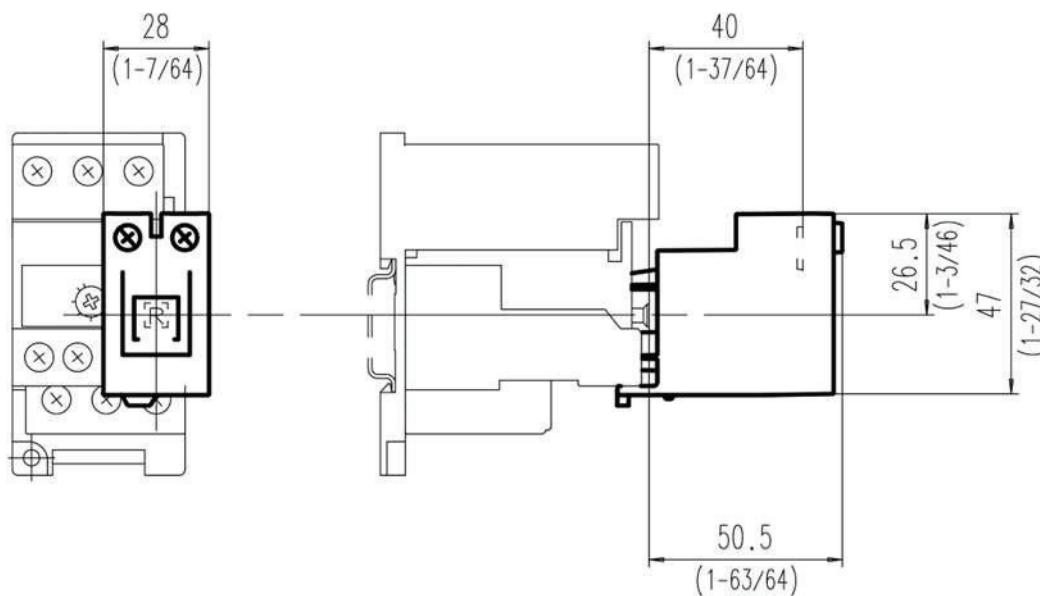
Dimension Diagram
