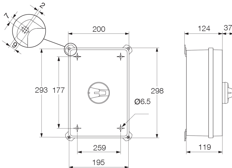
Dimension Diagram
