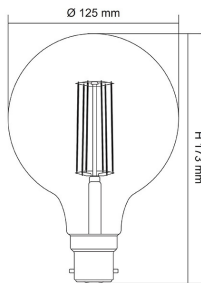
LG125 BC
