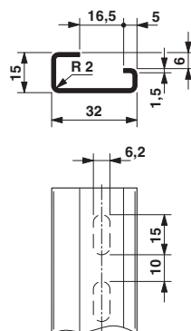
Dimensioned drawing
