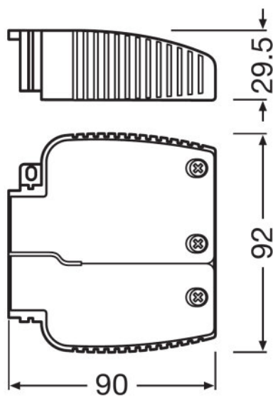
OT CABLE CLAMP B-STYLE TL
