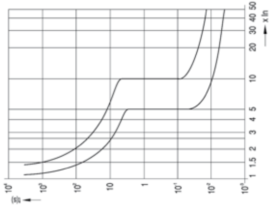
TRIPPING CURVE
