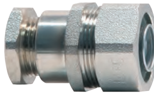
LC - SPS (IP66/67/68) Space Saver Multi part compression fitting with a nylon seal. Contains female threaded body component and a male threaded bush component, which minimises the amount of space taken up inside enclosures. Available in Brass (B)
