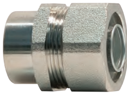
LC - FH - B (IP66/67/68) Internal Thread Female Hub fitting Multi part compression fitting with a nylon seal Available in Zinc Plated Steel, Nickel Plated Brass (B) and 316 Stainless Steel (SS)
