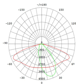
11201(50x150° ) 70W/90W
