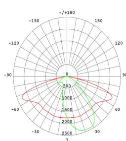
06302 (60x159° ) 20W/30W/50W
