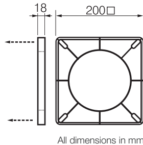
Spacer Plate (Model No: DPS150)
