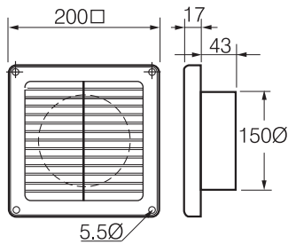
Slimfit Louvre Grille (Model No: DPL150)
