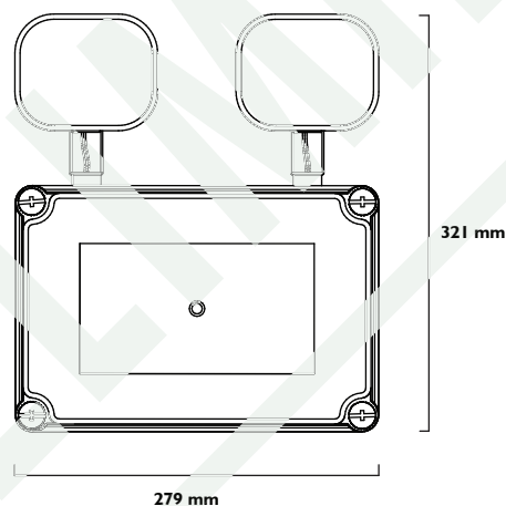
TWINSLOT LITE EMERGENCY IP65
