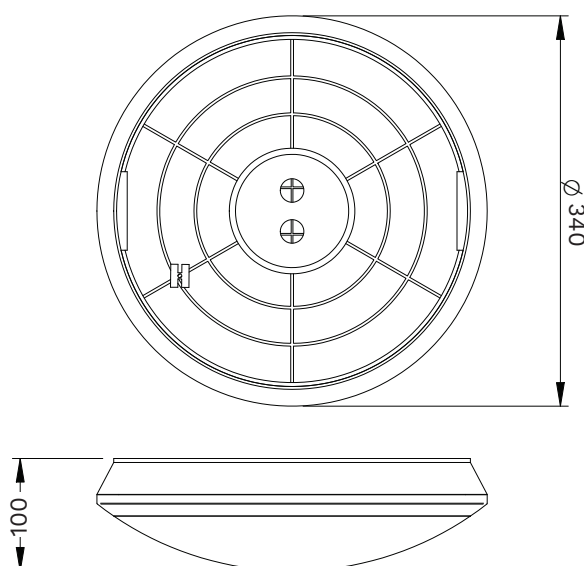
Dimensions (mm)
