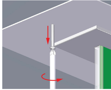
Pull down on screw whilst tightening to stop the Spring Toggle from spinning
