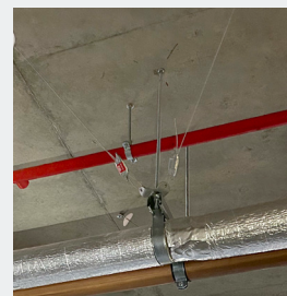
Seismic Bracing
